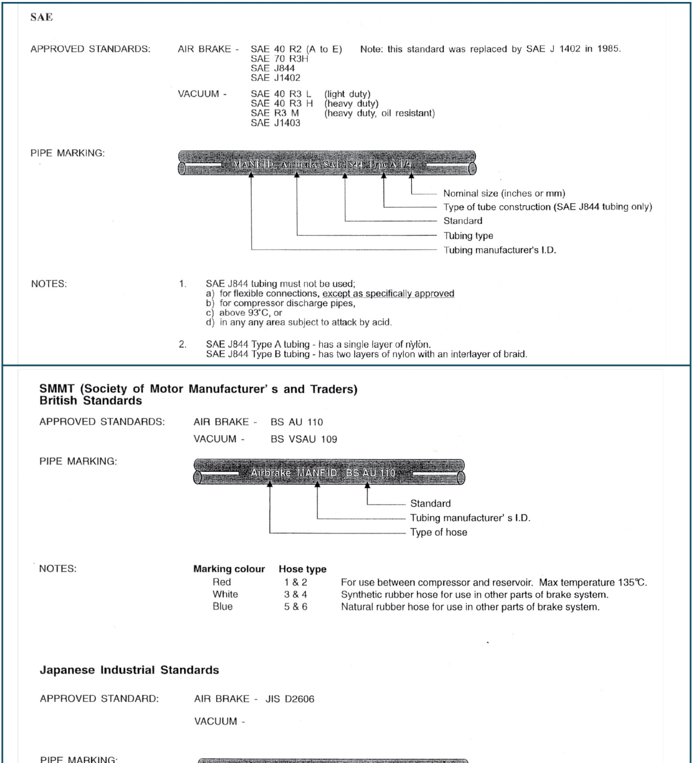
Figure 8-1-4. Brake hoses and flexible tubing information.
